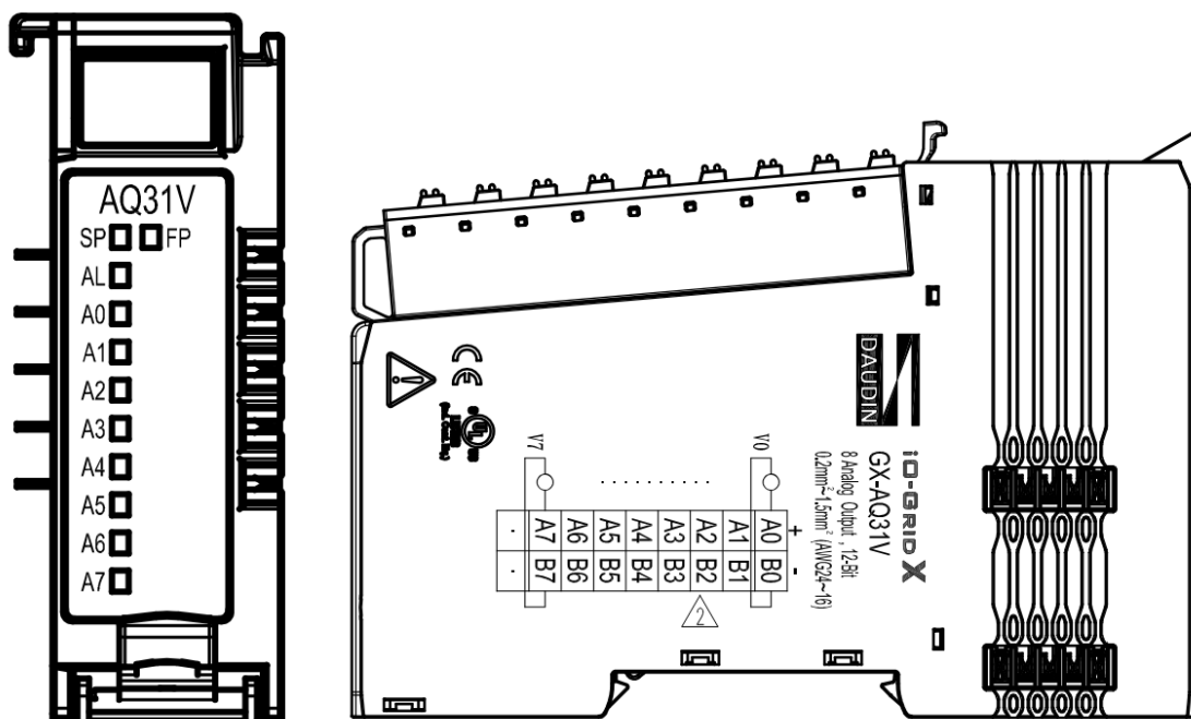
Figure 4.25 GX-AQ31V Wiring Diagram
