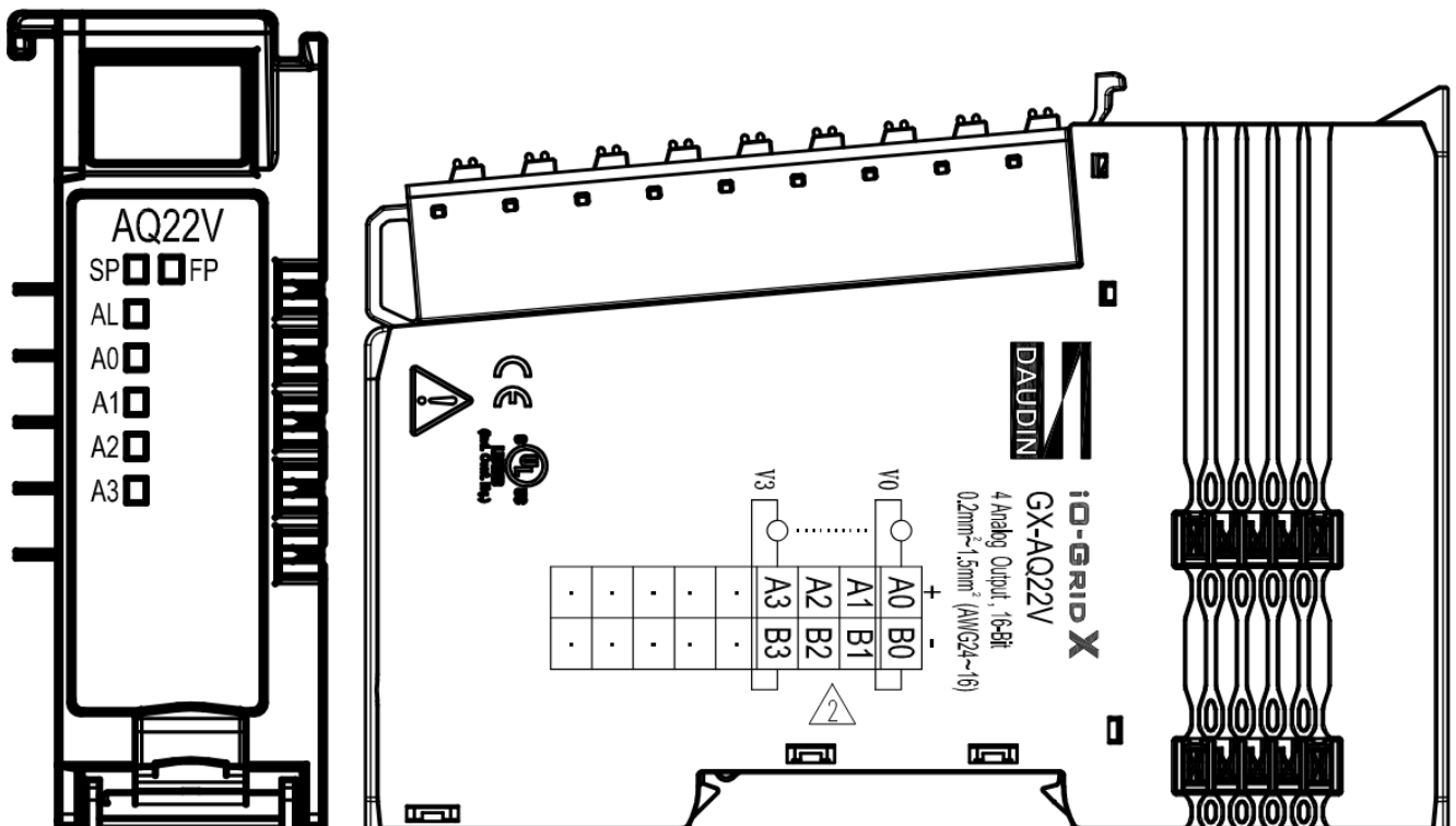
Figure 4.23 GX-AQ22V Wiring Diagram
