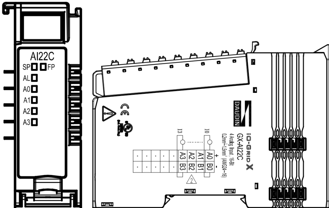
Figure 4.16 GX-AI22C Wiring Diagram
