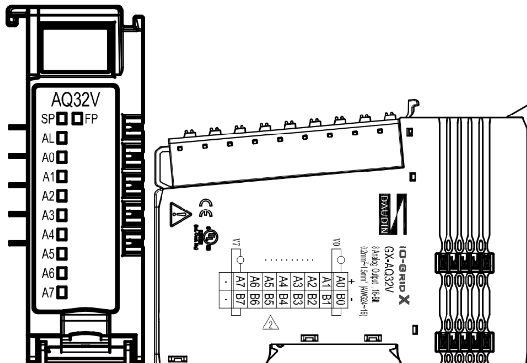
Figure 4.27 GX-AQ32V Wiring Diagram
