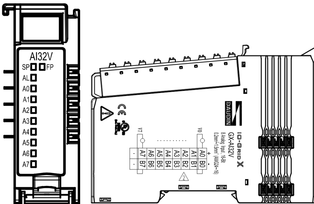
Figure 4.19 GX-AI32V Wiring Diagram
