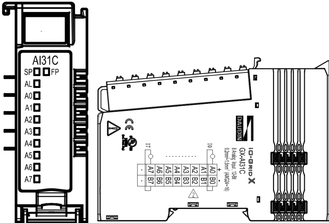
Figure 4.18 GX-AI31C Wiring Diagram
