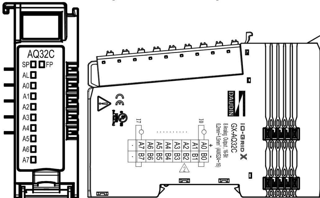
Figure 4.28 GX-AQ32C Wiring Diagram
