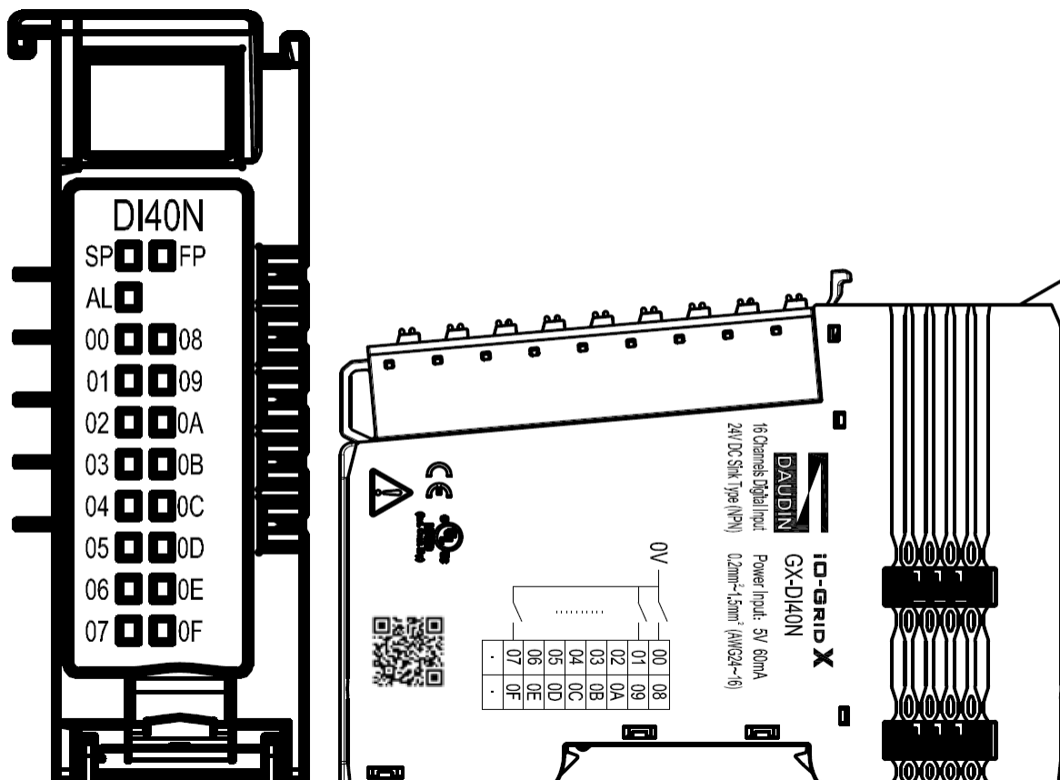
Figure 4.5 GX-DI40N Diagram
