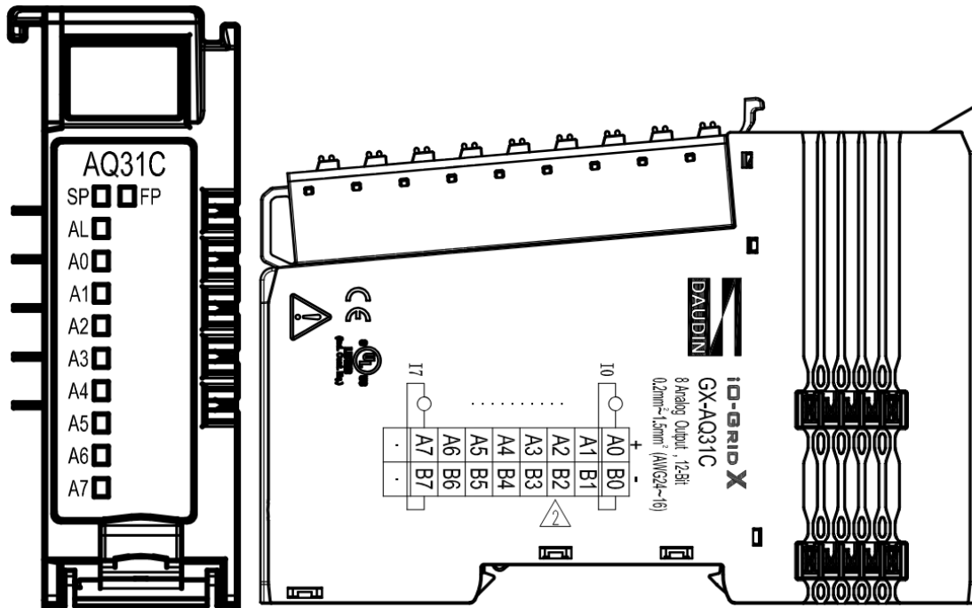
Figure 4.26 GX-AQ31C Wiring Diagram
