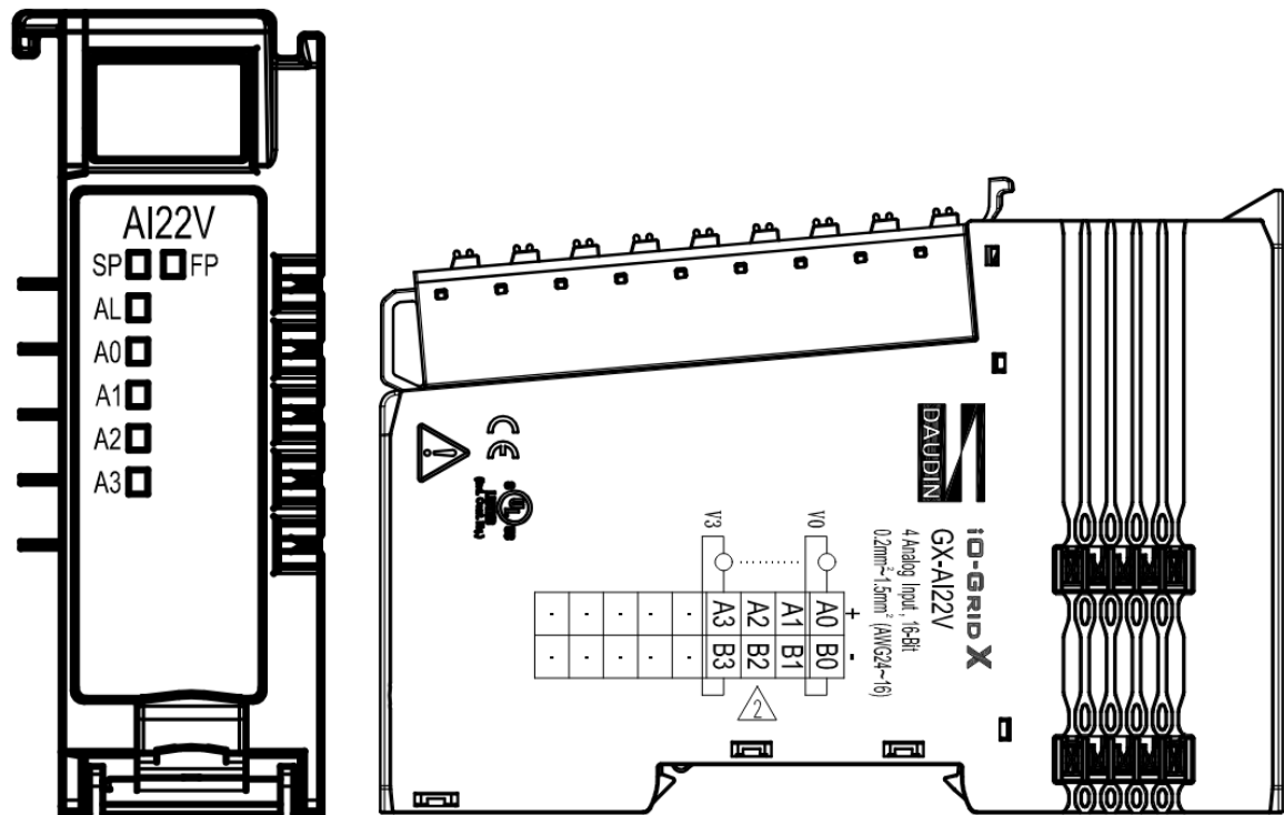
Figure 4.15 GX-AI22V Wiring Diagram
