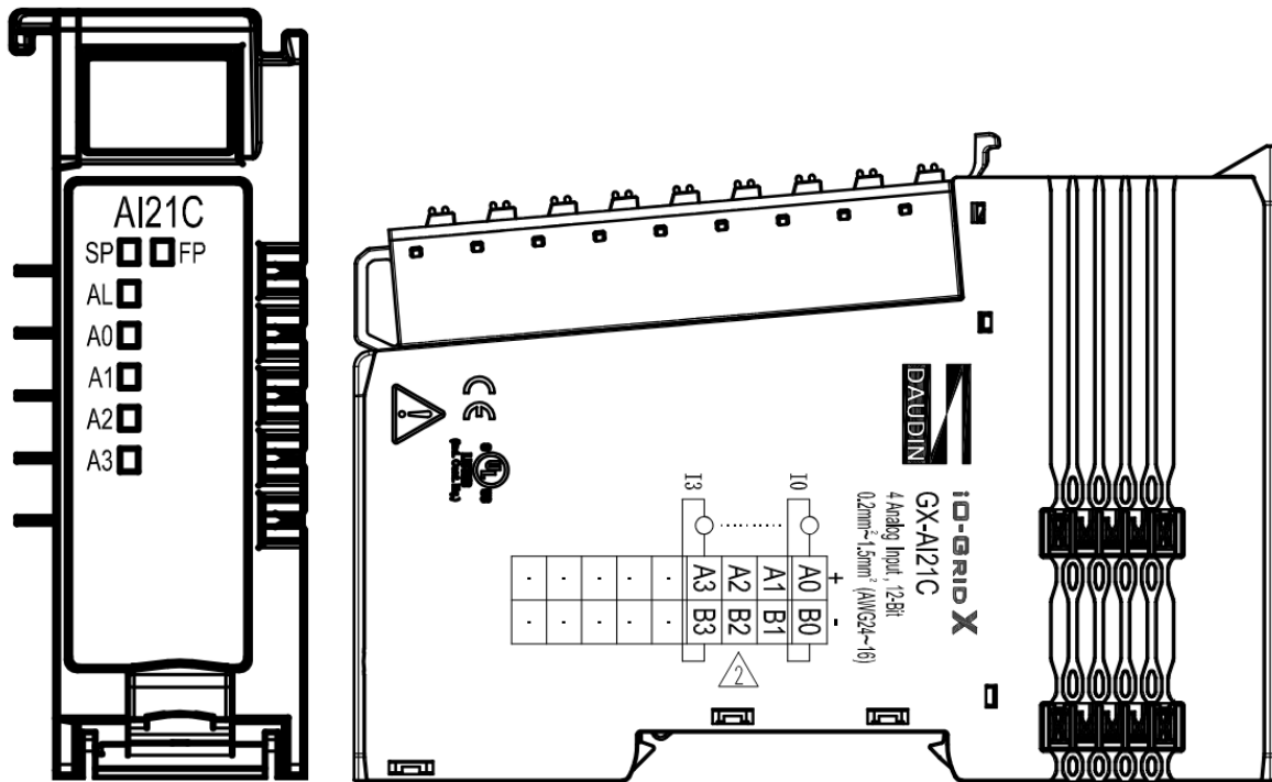
Figure 4.14 GX-AI21C Wiring Diagram
