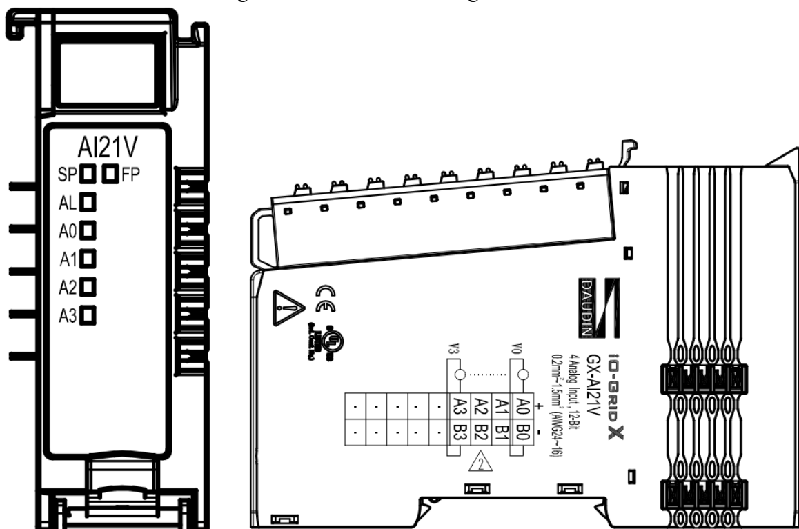
Figure 4.13 GX-AI21V Wiring Diagram
