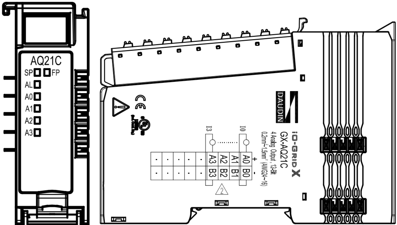
Figure 4.22 GX-AQ21C Wiring Diagram
