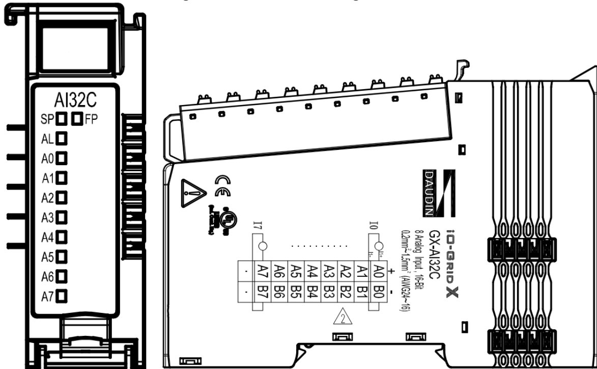
Figure 4.20 GX-AI32C Wiring Diagram
