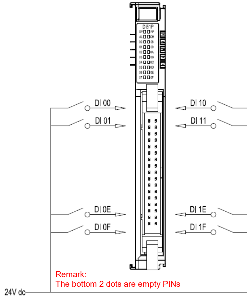
Field Power Supply Figure 8.7 GX-DI51P Wiring Diagram
